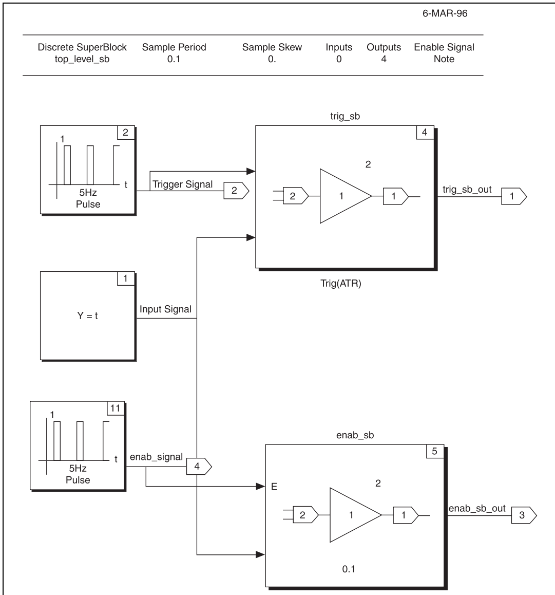
Figure 8-1. Model with Enabled and Triggered Tasks
